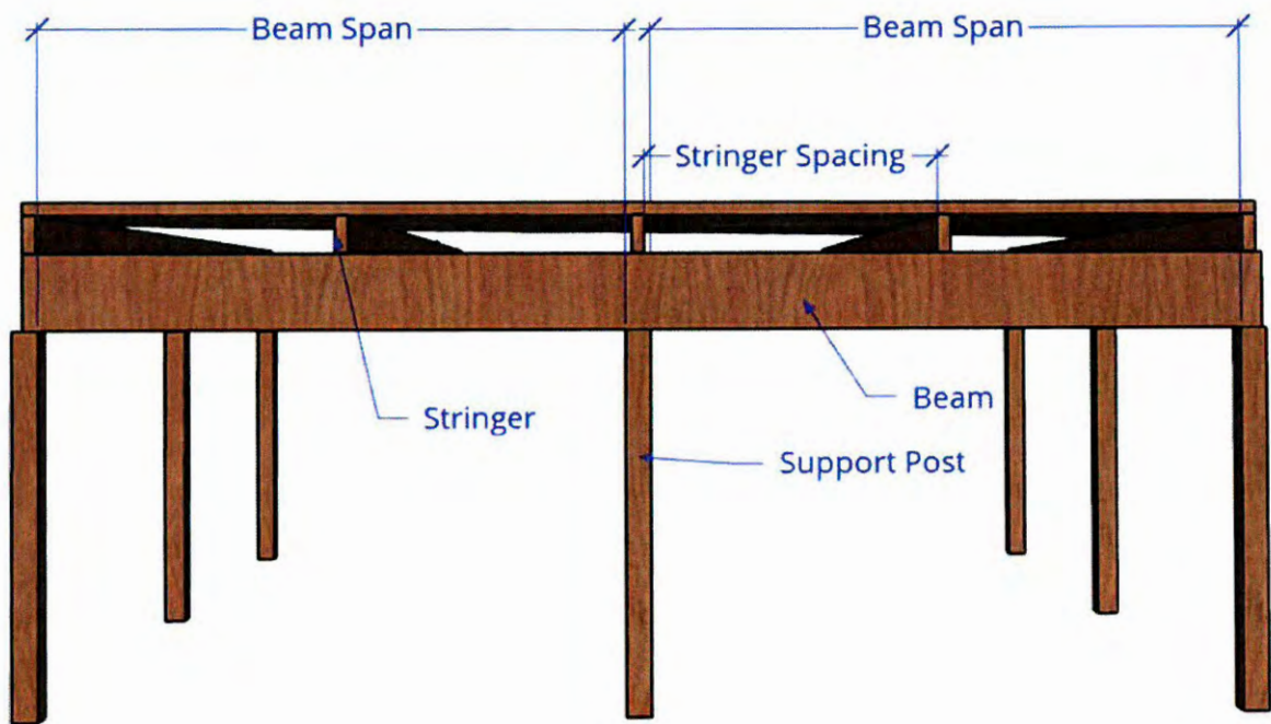
Figure 2: Beam Span
