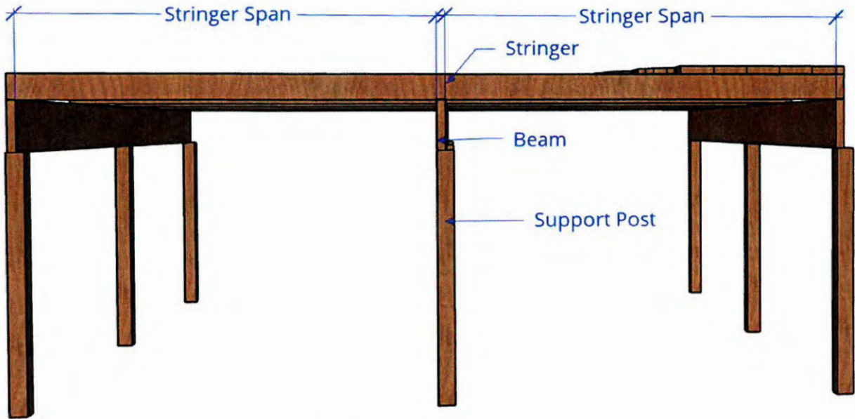
Figure 1: Stringer Span
