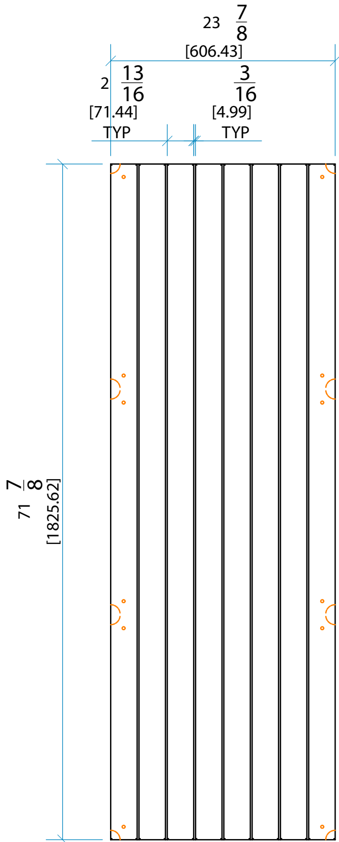
TOP VIEW
